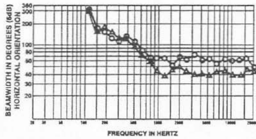
FIGURE 5 — Directivity vs. Frequency
