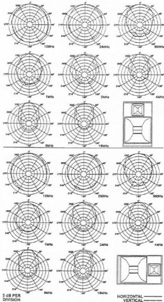
FIGURE 3 — Polar Response
