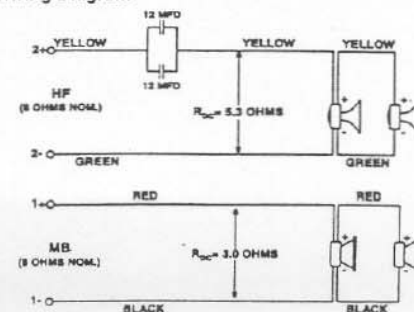
FIGURE 7 — Wiring Diagram
