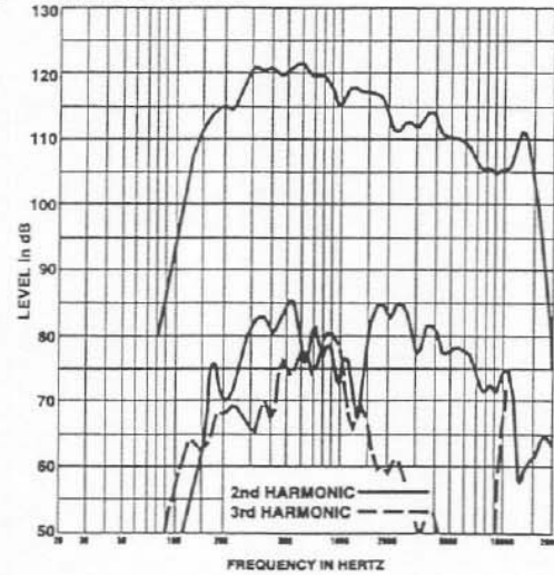
FIGURE 6 — Harmonic Distortion
